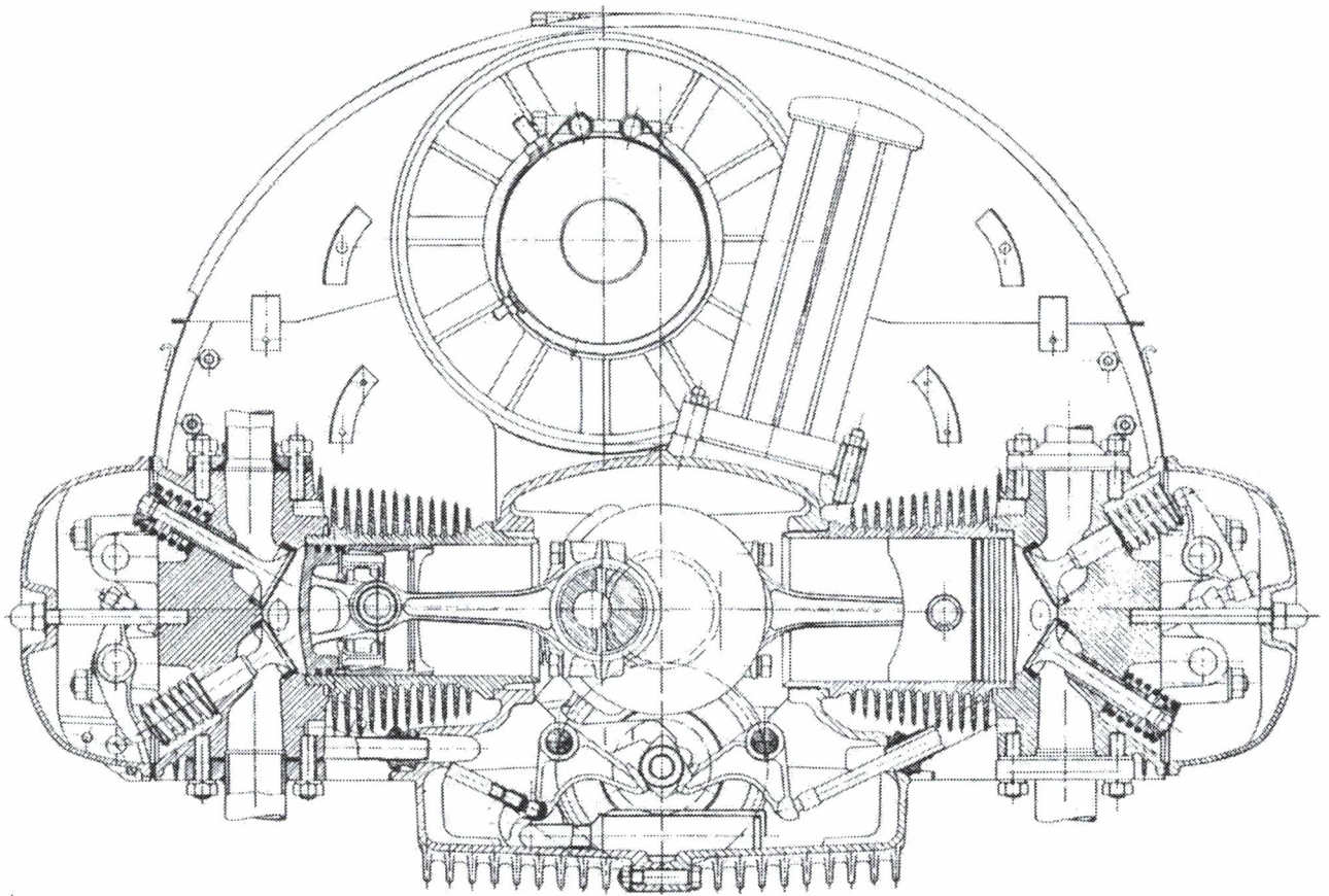
Haflinger-Motor.
